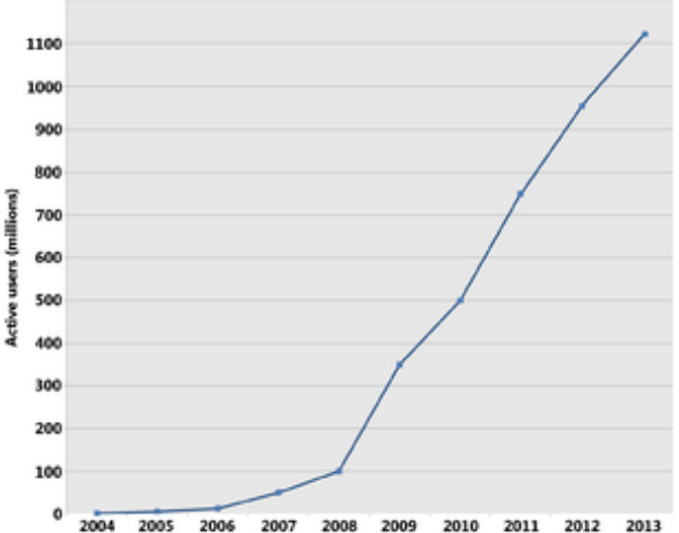
Facebook - popularity
